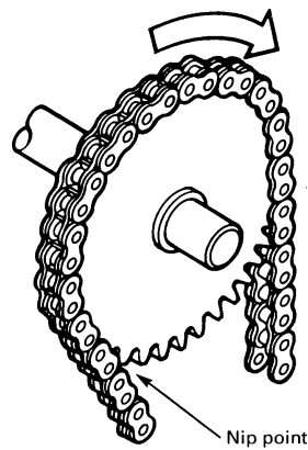
FIG. 2 ROTATING MOTION
